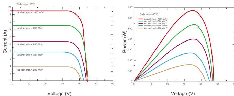
Current-Voltage & Power-Voltage Curves (RMH66-670S2)
