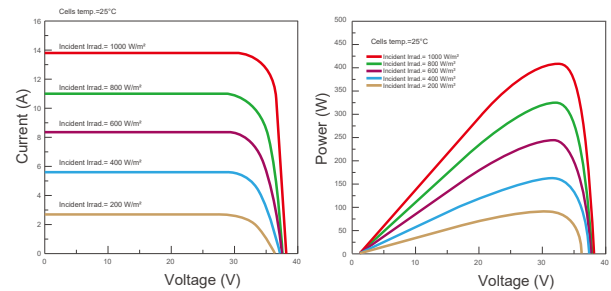
Current-Voltage & Power-Voltage Curves (RMHT54/405O2)
