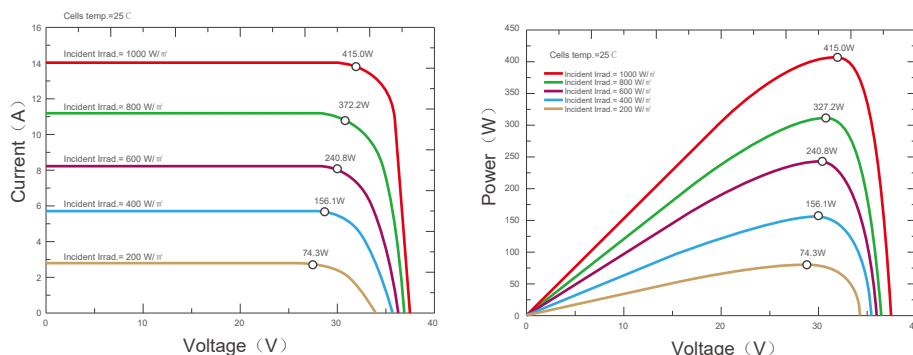
Current-Voltage & Power-Voltage Curves (RMHB54-415AB2)
