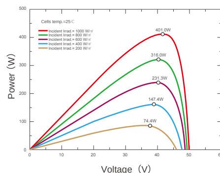
Current-Voltage & Power-Voltage Curves (RMH72-400AB1)
