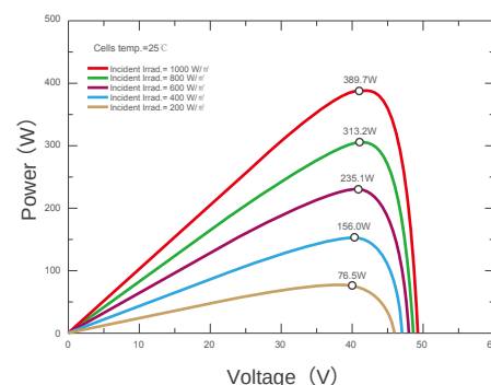
Current-Voltage &amp; Power-Voltage Curves (RM72-385S1)
